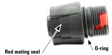
Plug
