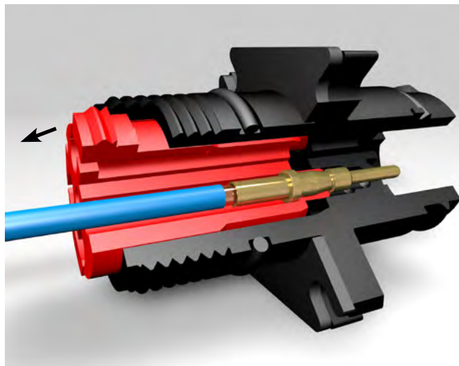
Unlocked plate
